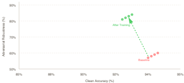
Robustness-Accuracy Trade-off
