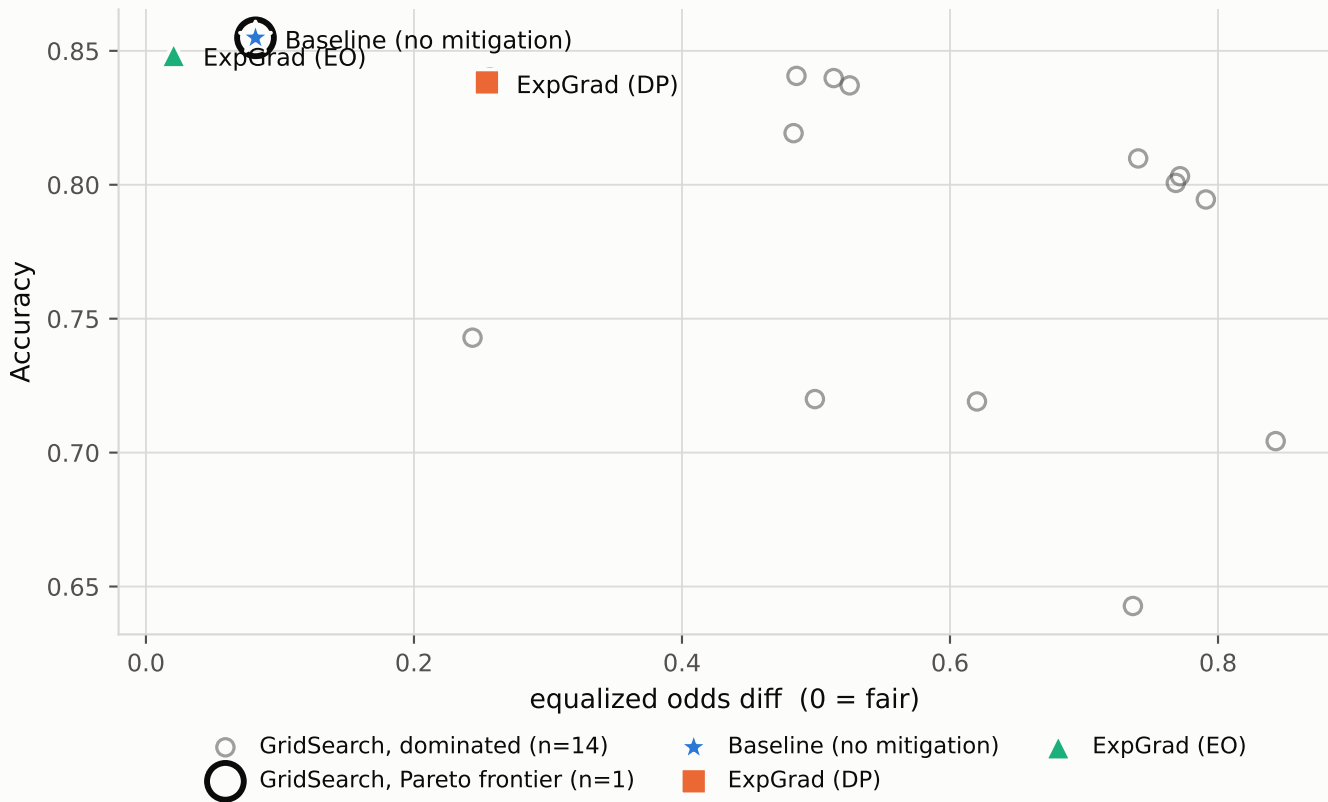
Accuracy vs fairness on Adult: GridSearch frontier decision tree (depth 8), single split — up and to the left is better
