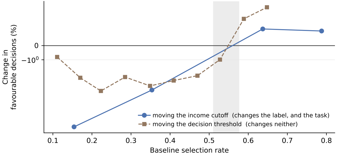
Fig. 2. The design that separates the selection rate from the difficulty of the task. Moving the income cutoff changes the label, and therefore how hard the problem is; moving the decision threshold changes neither, only where the fitted model draws its line. Both routes cross zero inside the same band. If difficulty were doing the work, the second curve would not reproduce the first.
