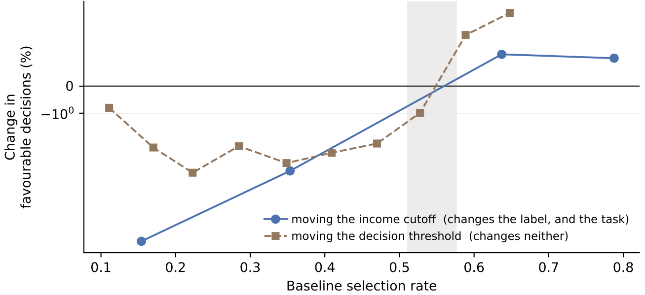
Fig. 2. The design that separates the selection rate from the difficulty of the task. Moving the income cutoff changes the label, and therefore how hard the problem is; moving the decision threshold changes neither, only where the fitted model draws its line. Both routes cross zero inside the same band. If difficulty were doing the work, the second curve would not reproduce the first.
