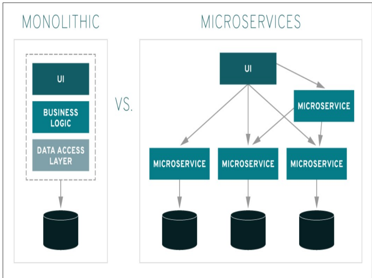
FIGURE 2.7 – Architecture monolithique versus architecture microservices
