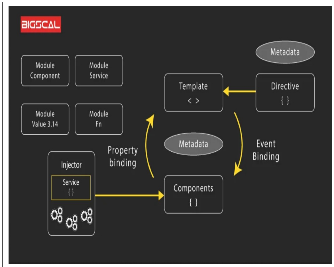
FIGURE 2.4 – Architecture logique Front-End (Angular)
