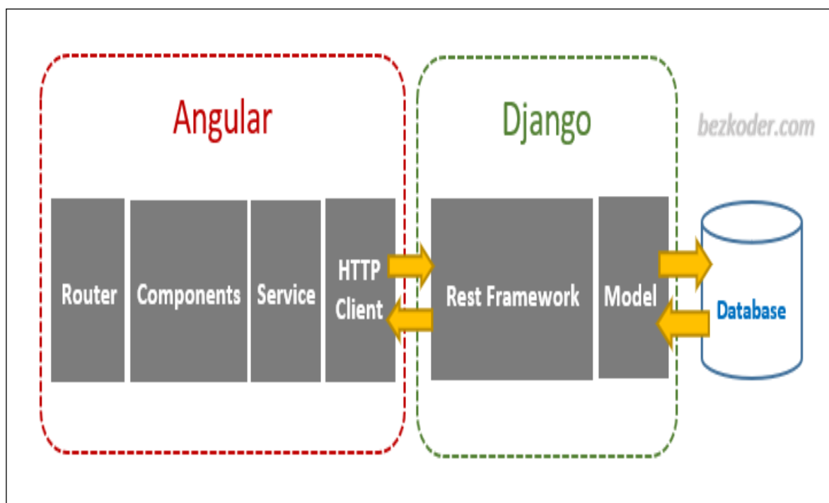
FIGURE 2.3 – Architecture logique de l'application
