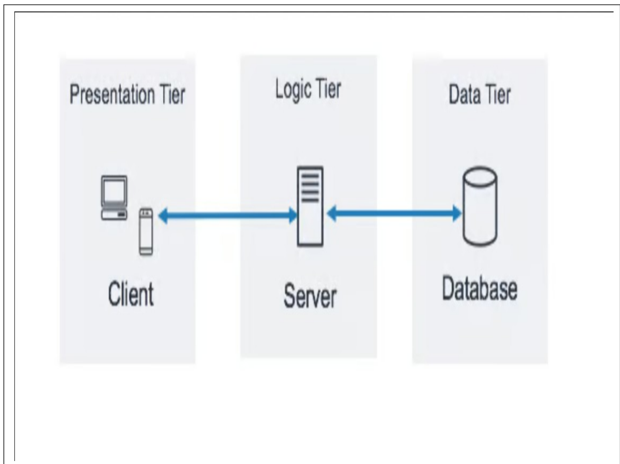
FIGURE 2.6 – Architecture physique globale
