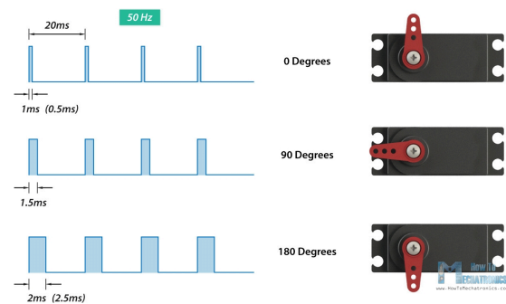
Figure 31: PWM pulse width controlling servo motor angle.
