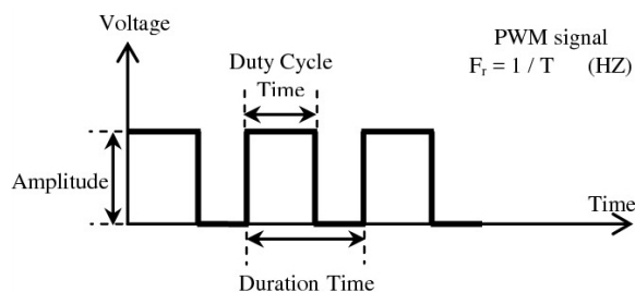
Figure 30: Basic representation of a PWM signal and its parameters.
