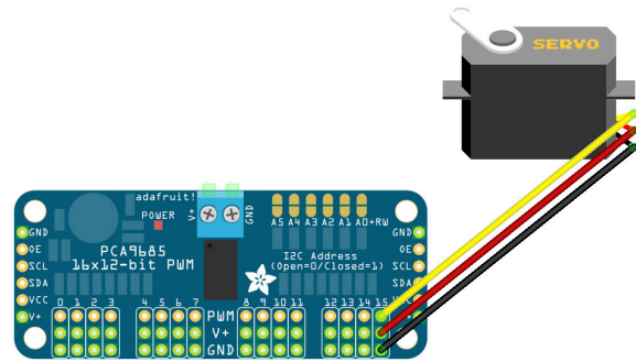
Figure 39: Connecting a servo motor to a channel of the PCA9685 module.
