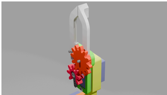
Figure 37: Mechanical Assembly — Step 5: End-Effector with Gear Mechanism.
