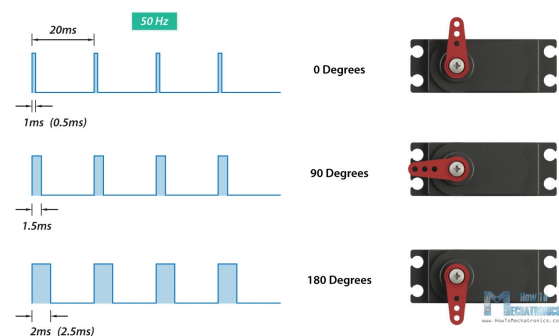
Figure 30: PWM pulse width controlling servo motor angle.
