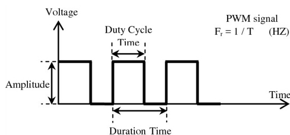
Figure 29: Basic representation of a PWM signal and its parameters.
