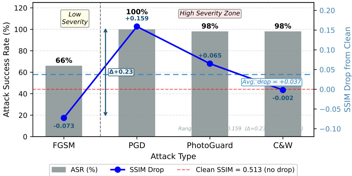
Attack Severity: ASR and Perceptual Degradation (COCO-50)
