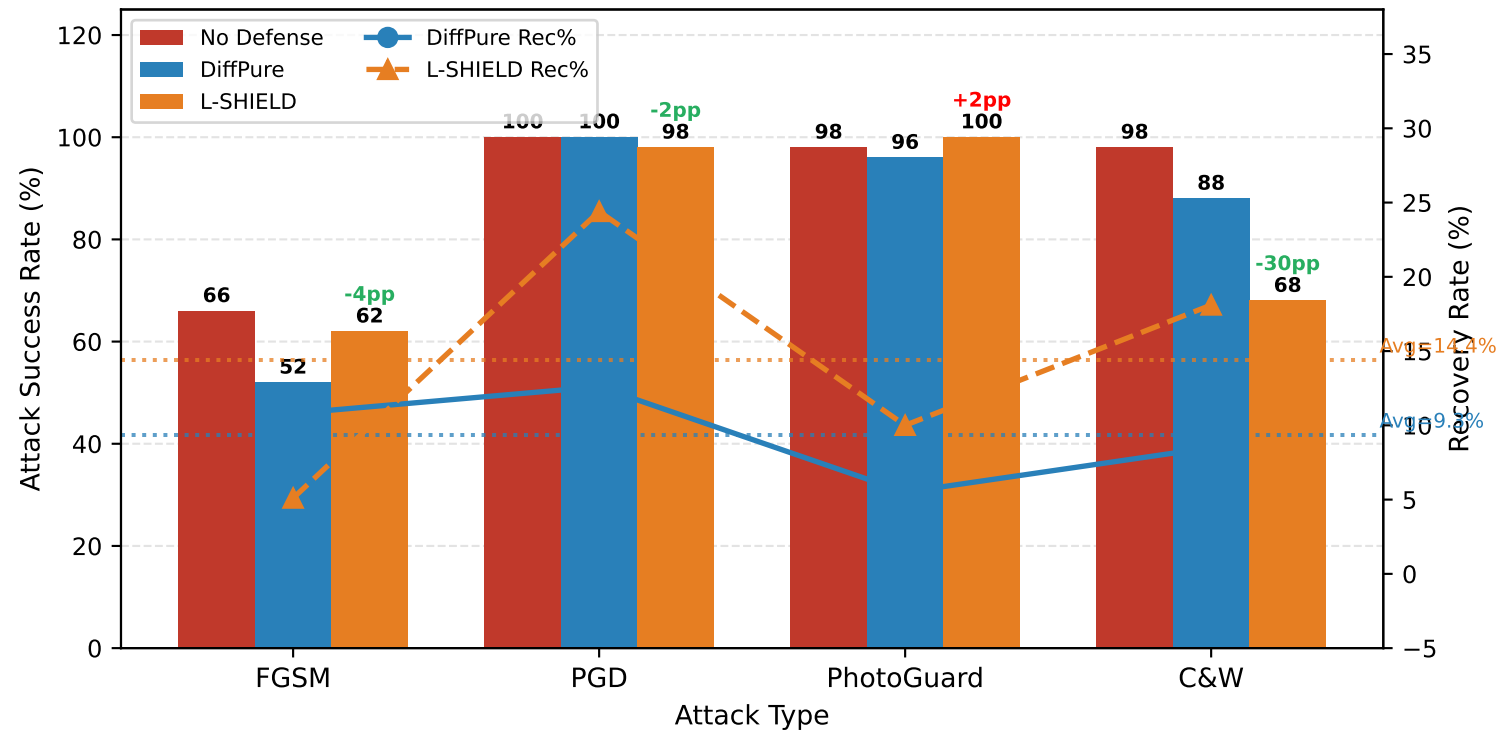
Defense Comparison: ASR Reduction and Recovery Rate (COCO-50)
