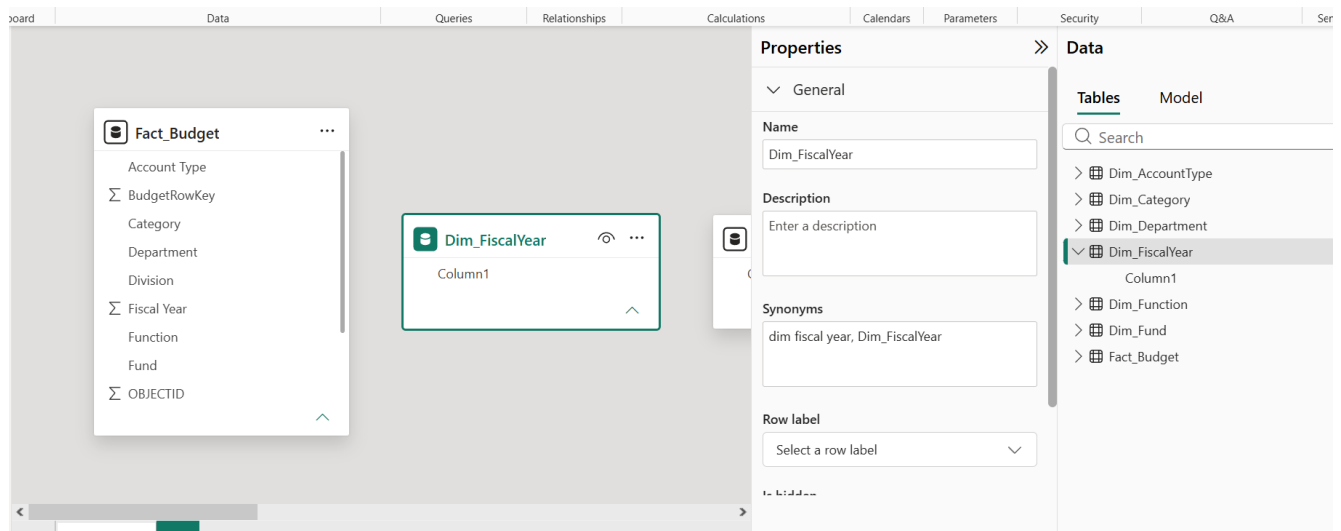
Figure 12. User-provided Power BI model screenshot showing Fact_Budget and dimension tables.
