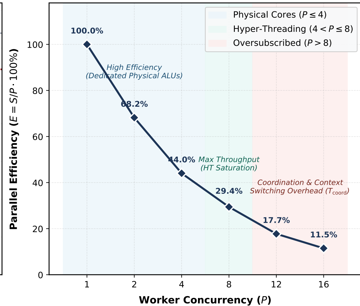
(c) Parallel Efficiency & Hardware Regimes
