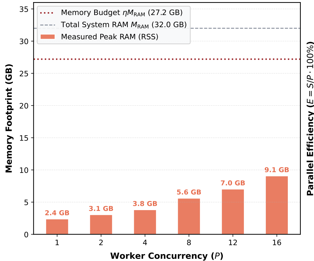
(b) Peak Memory Footprint & Safety Margin
