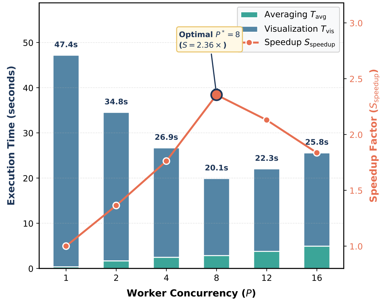
(a) Execution Time Breakdown & Speedup
