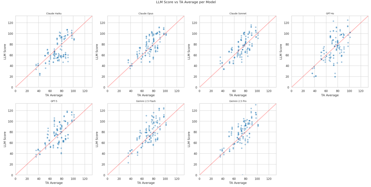
Figure 1: Figure 1. . Per-model scatter of model score against TA consensus.
