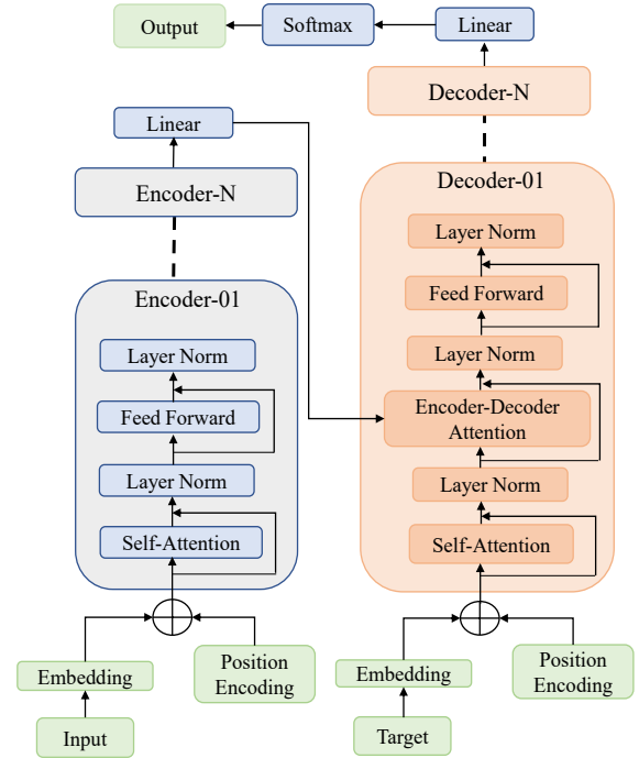
Fig. 1. Transformer Architecture.
