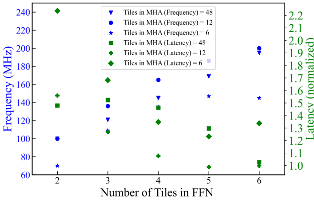
Fig. 7. Choosing the optimum tile size.
