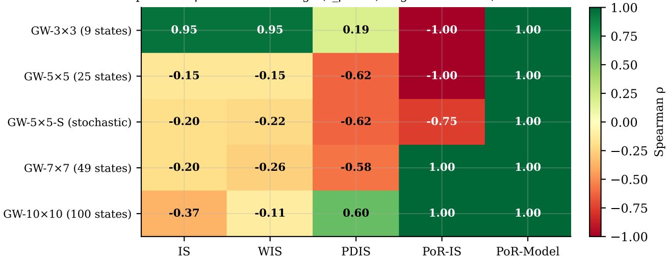
Spearman \rho at worst coverage ( \varepsilon_\beta=0.9 ) — green=correct, red=reversed
