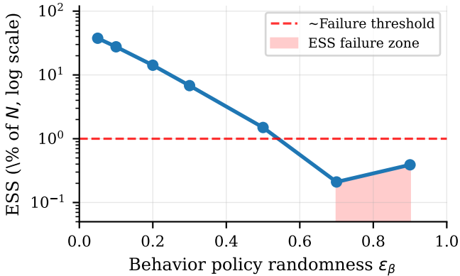
(a) ESS collapses as behavior diverges from target policy
