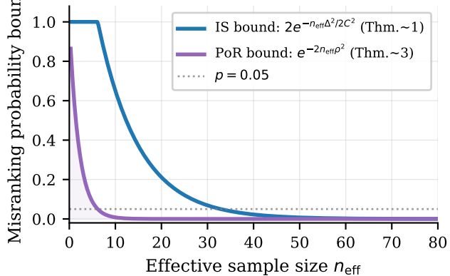
(b) PoR bound tighter than IS bound (no C dependence \Rightarrow robust to heavy tails)
