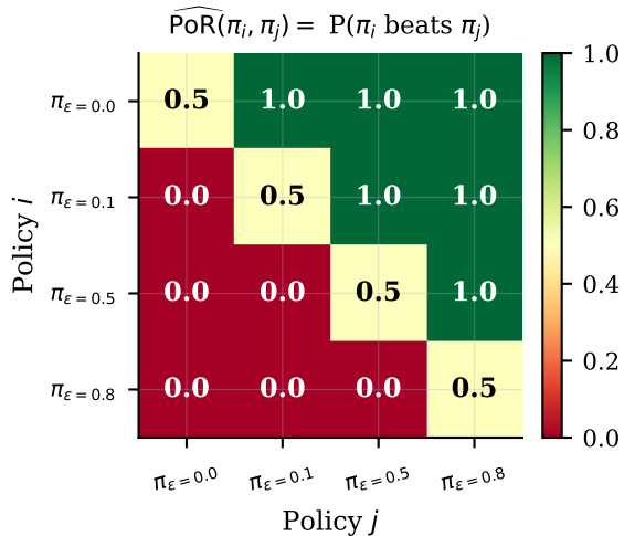
(b) PoR-Model matrix — S2 (ESS=0.1\%)
