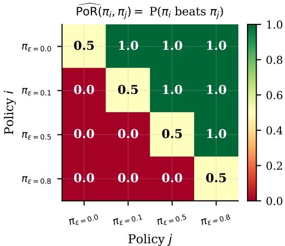
(a) PoR-Model matrix — S1 (ESS=11.2\%)
