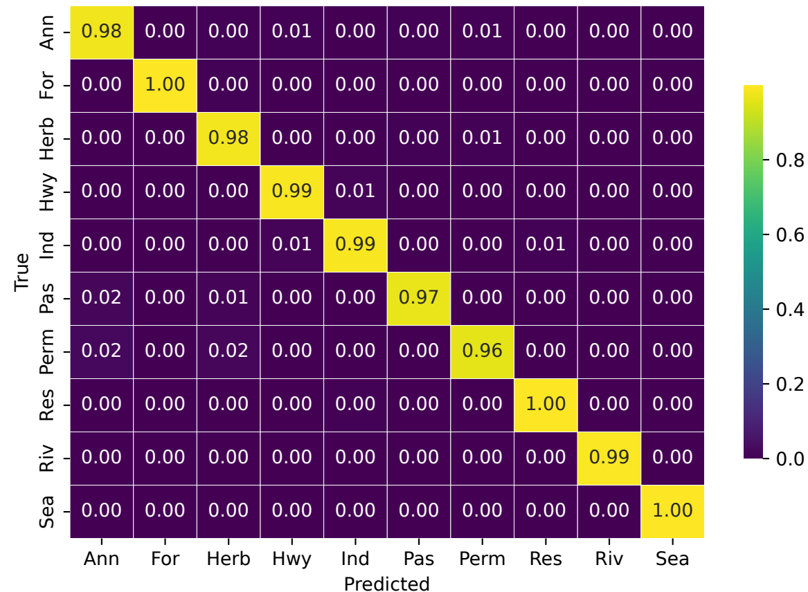
EXP-D — Dual 4+4 VQC (proposed) (OA=0.9713)
