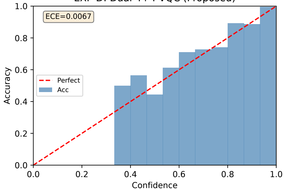
EXP-D: Dual 4+4 VQC (Proposed)
