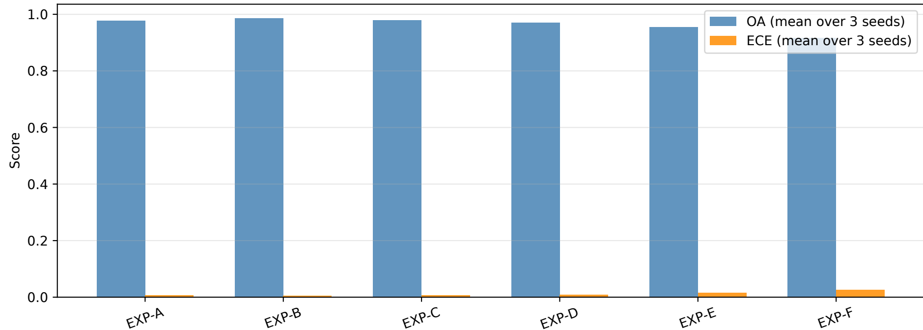
Overall Accuracy and ECE — All Experiments
