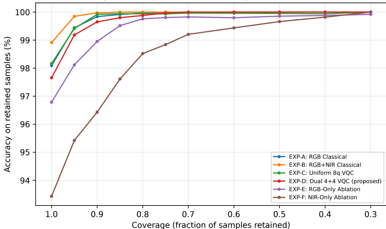
Risk-coverage: does epistemic uncertainty enable useful abstention?
