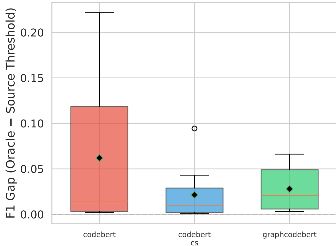
(a) Threshold Transfer Gap by Model
