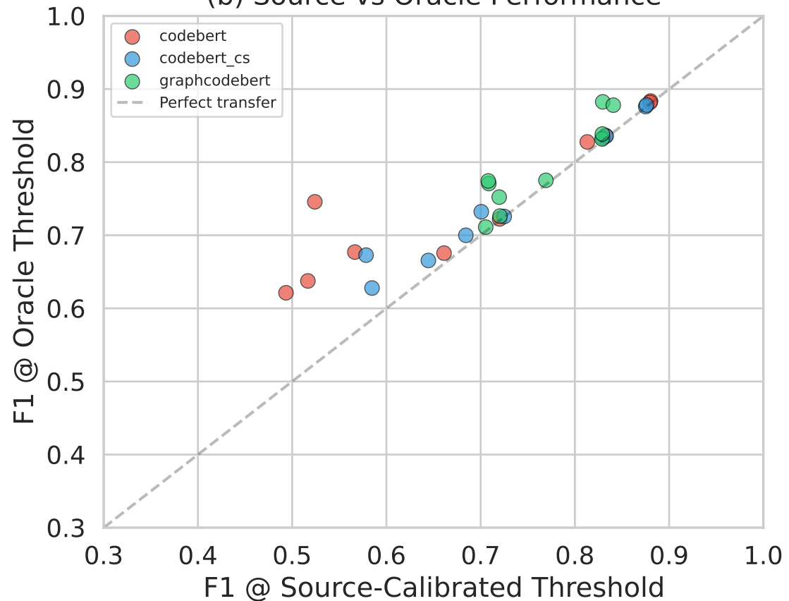
(b) Source vs Oracle Performance
