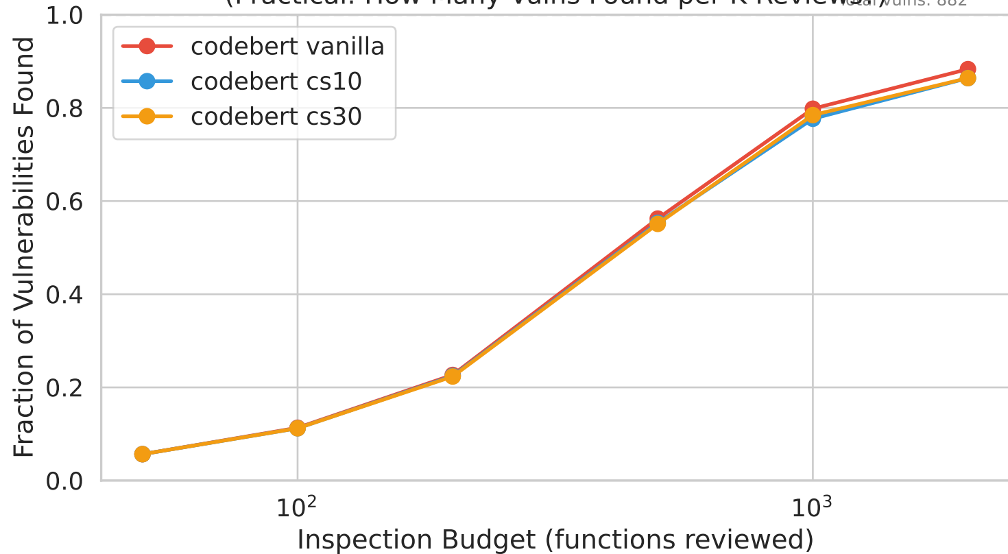
Budget-Constrained Vulnerability Detection (Practical: How Many Vulns Found per K Reviews?)
