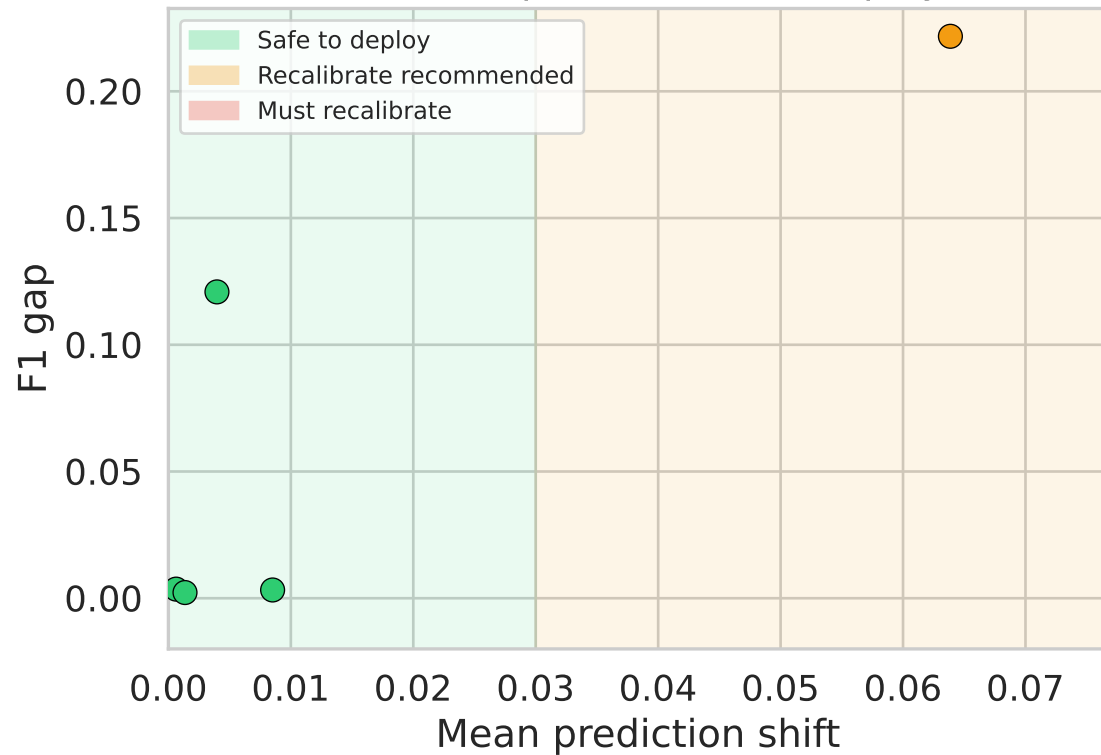
(b) Deployment risk zones (label-free, computable before deployment)
