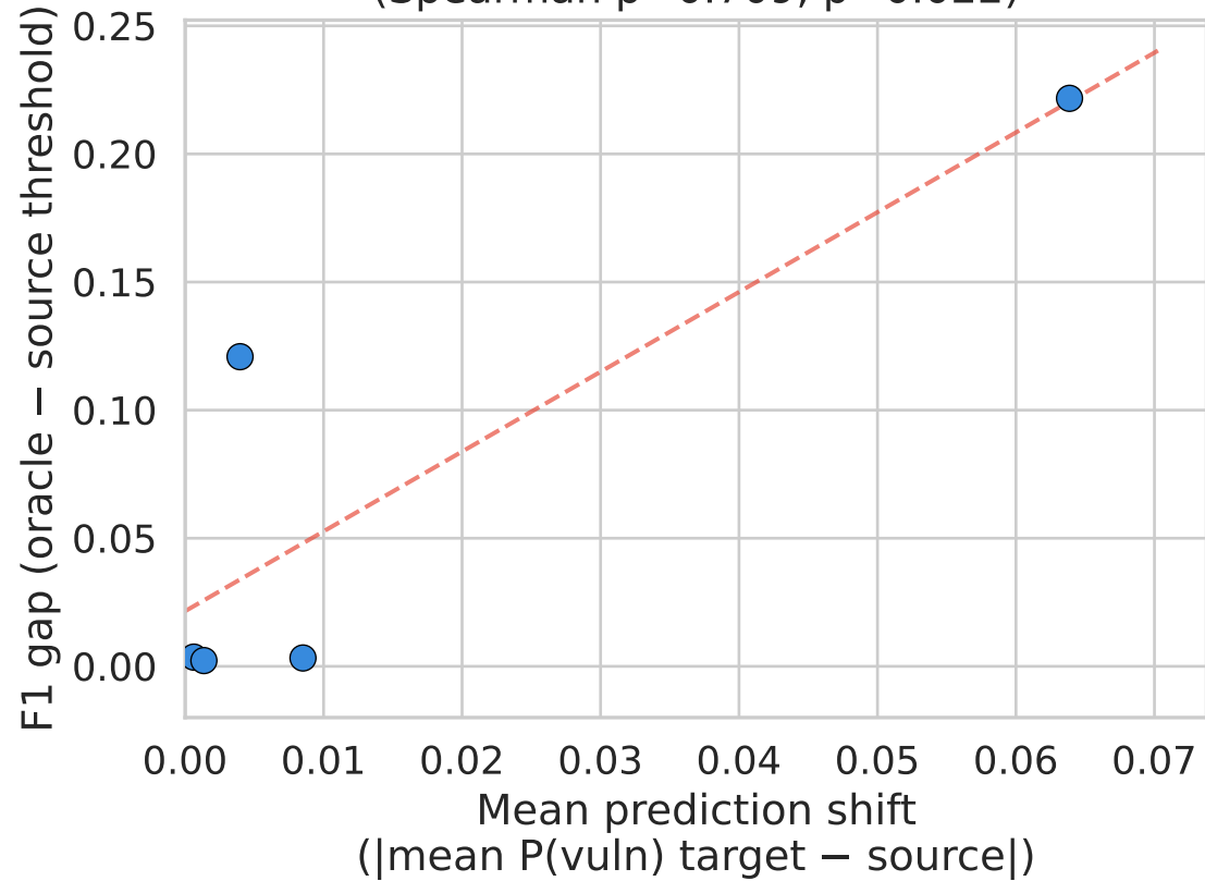
(a) Prediction shift predicts transfer failure (Spearman \rho=0.709 , p=0.022 )
