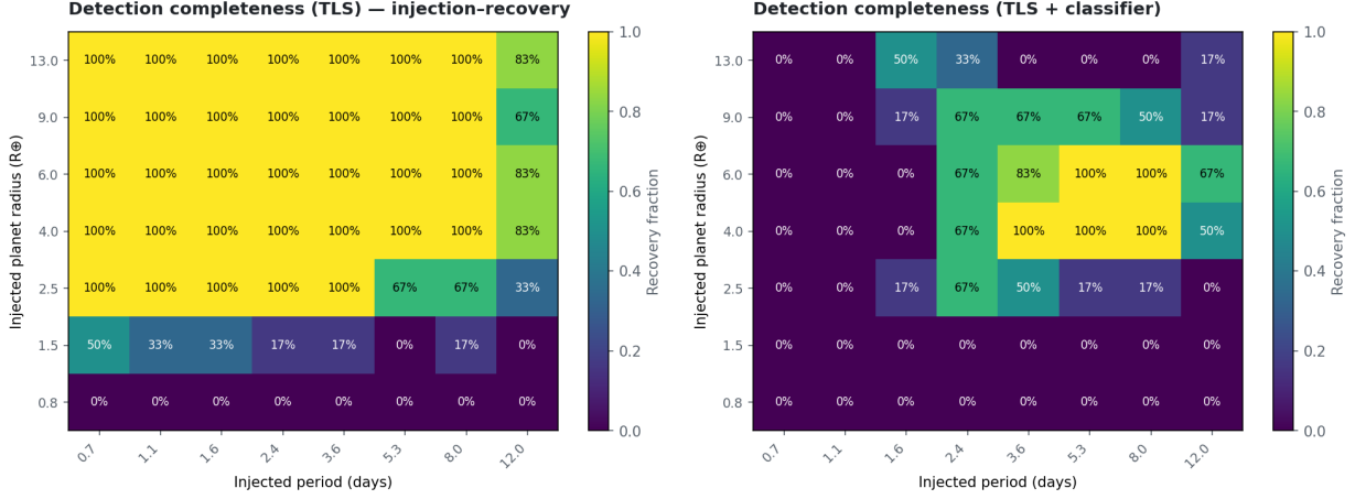
Figure 1: Detection completeness over injected period and radius: TLS recovery (left) and TLS+classifier recovery (right). The classifier suppresses the giant-radius corner because such depths are EB-like.
