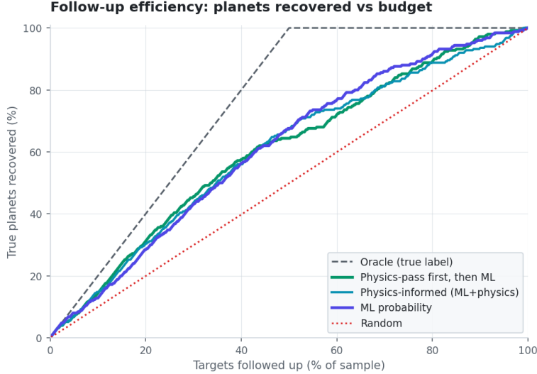
Figure 7: Follow-up efficiency: cumulative true planets recovered vs. fraction of targets observed. At n = 500 the physics-informed and probability rankings coincide; both beat random and trail the oracle.
