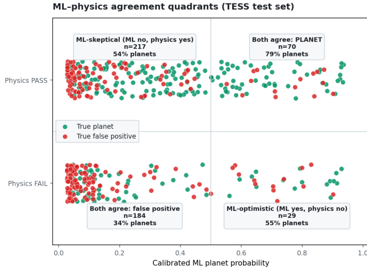
Figure 6: ML–physics agreement quadrants on the TESS test set; box annotations give the count and true-planet purity per quadrant.
