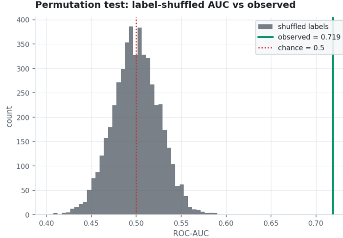
Figure 8: Permutation test: the observed cross-mission AUC lies far outside the label-shuffled null distribution, so the signal is not a metric artifact.
