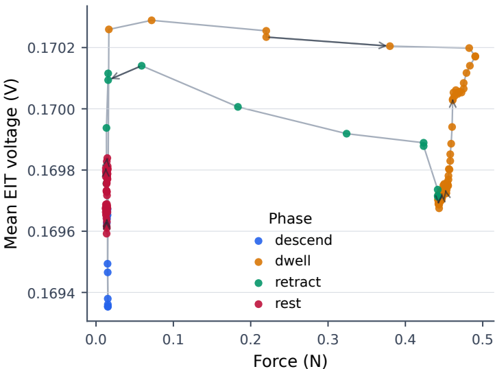
Force vs mean EIT, batch 70
