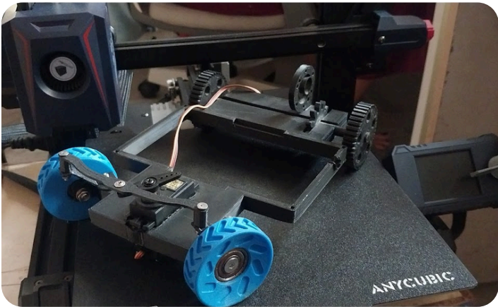
Revised prototype WRO vehicle chassis
