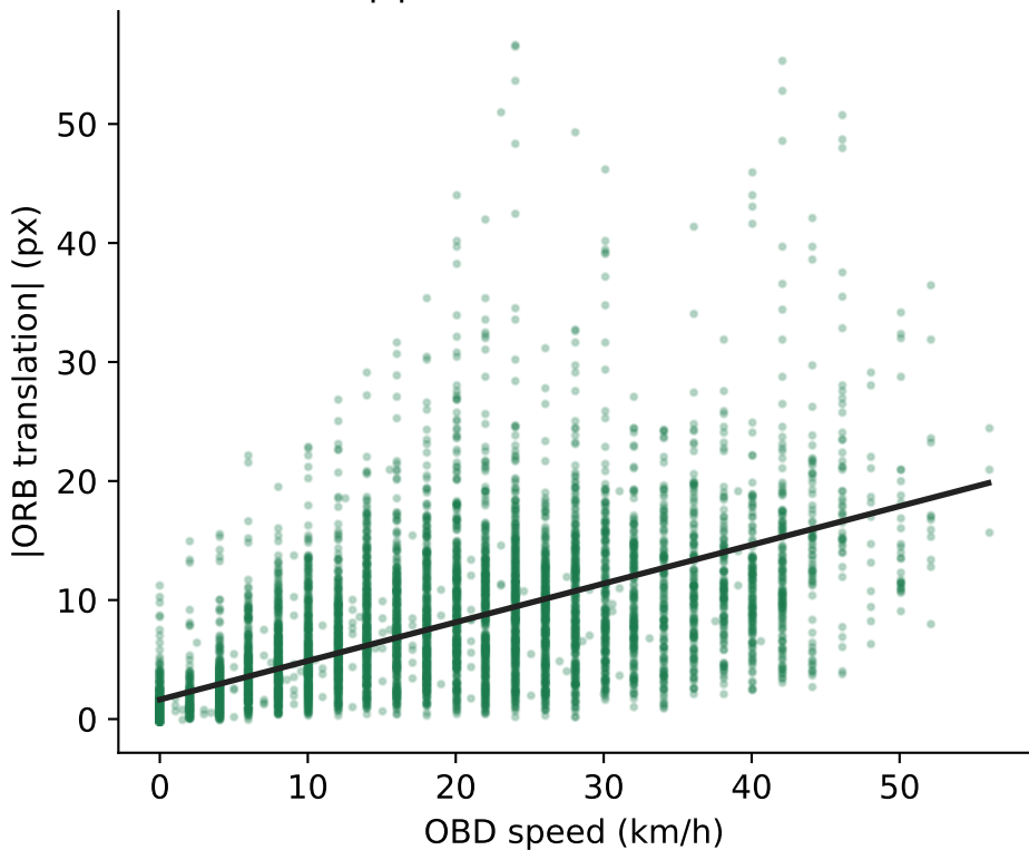
ORB affine |t| vs OBD ( R^2=0.413 , n=75268 )
