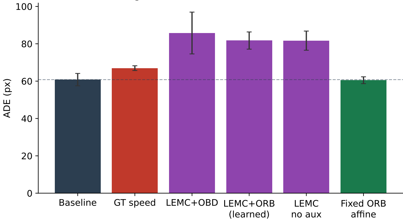
Main grid — PIE test (mean \pm std, 3 seeds)
