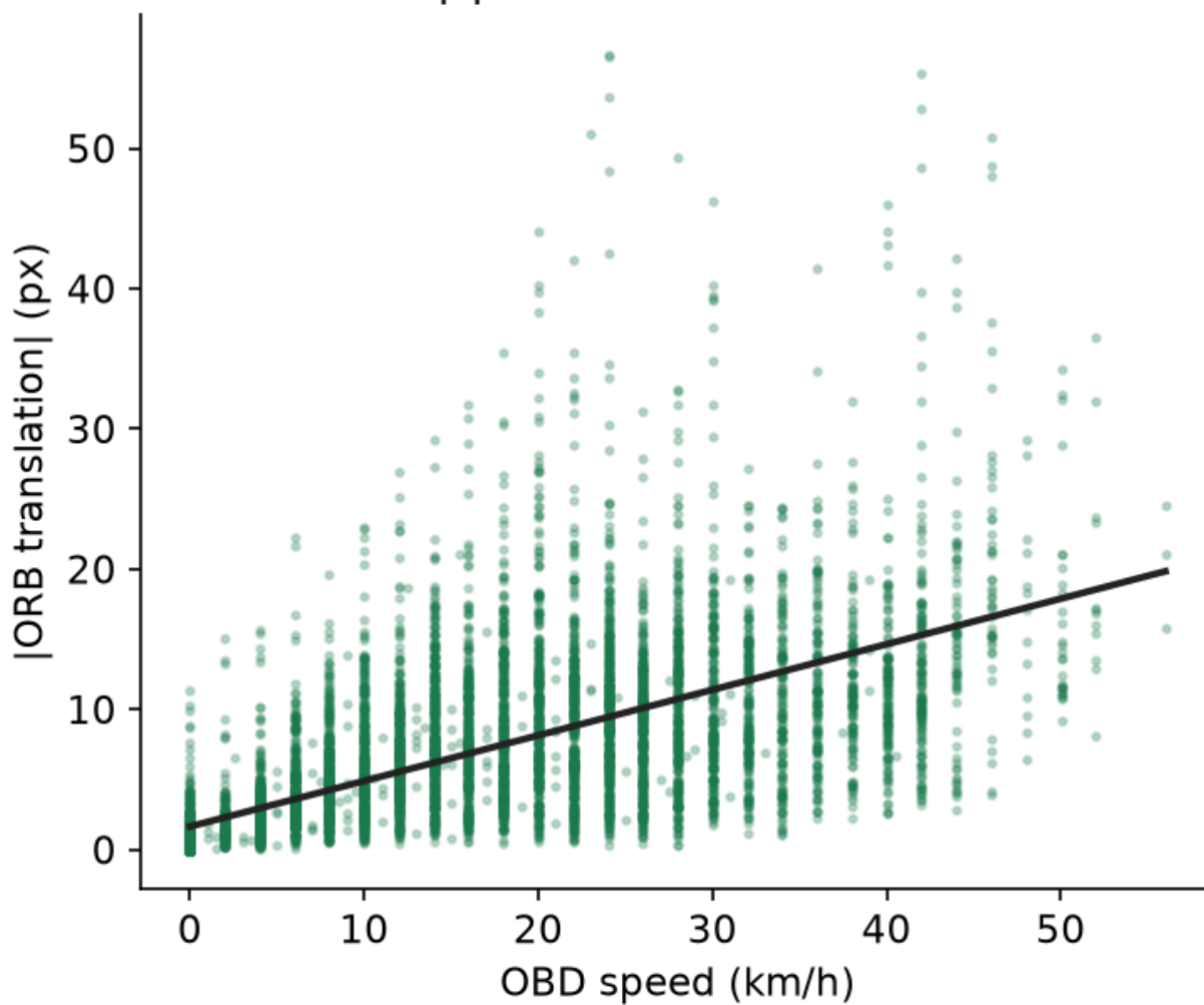
ORB affine |t| vs OBD ( R^2=0.413 , n=75268 )
