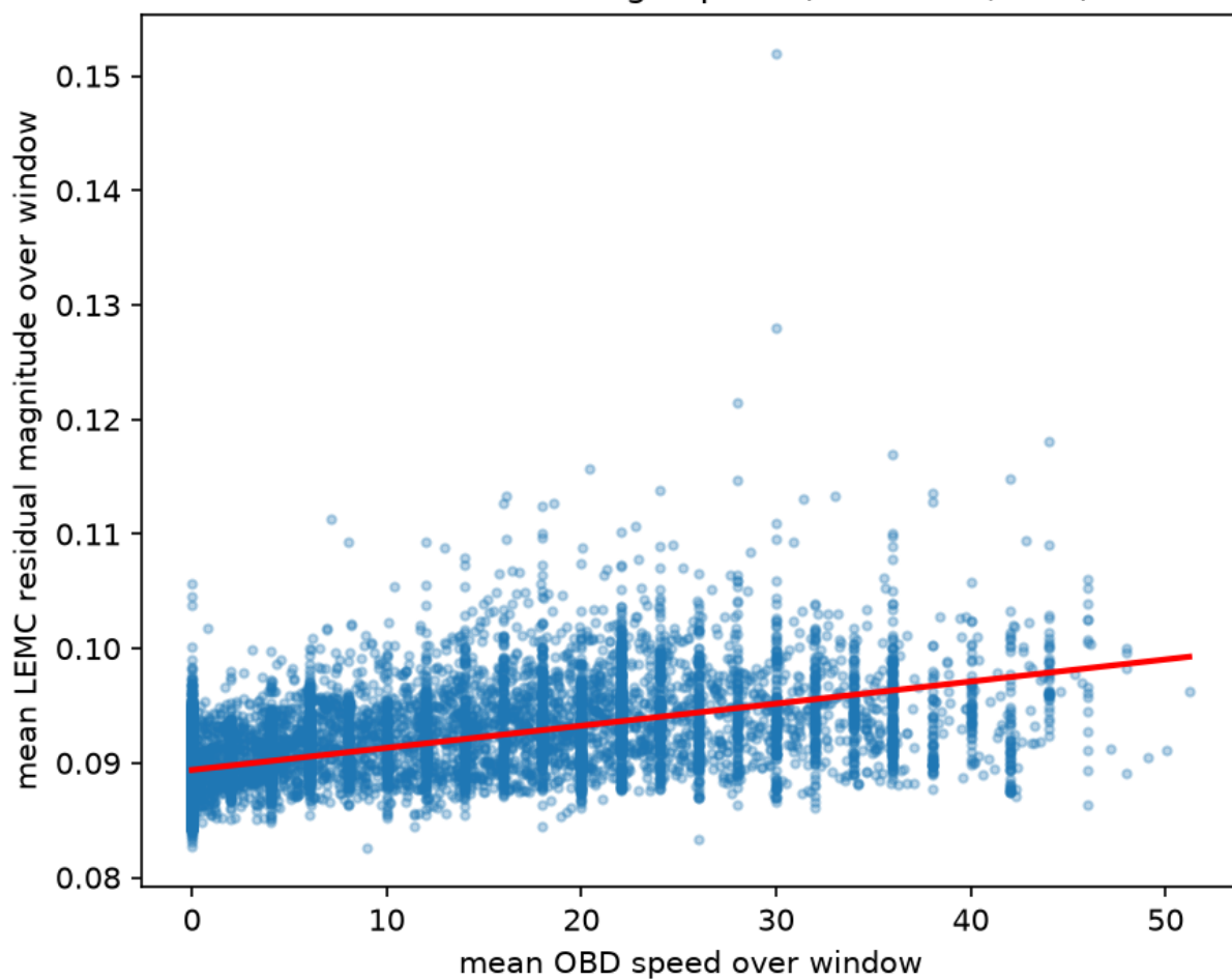
LEMC residual vs ego speed ( R^2=0.297 , test)
