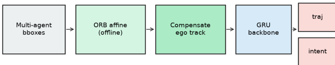
Fixed ORB-affine compensation (sensor-free at inference)
