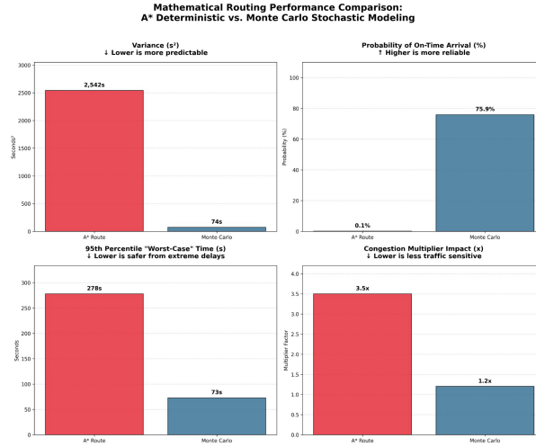
Figure 1: Performance comparison between A* deterministic routing and Monte Carlo stochastic modeling in terms of variance, on-time arrival probability, worst-case travel time (95th percentile), and congestion sensitivity.
