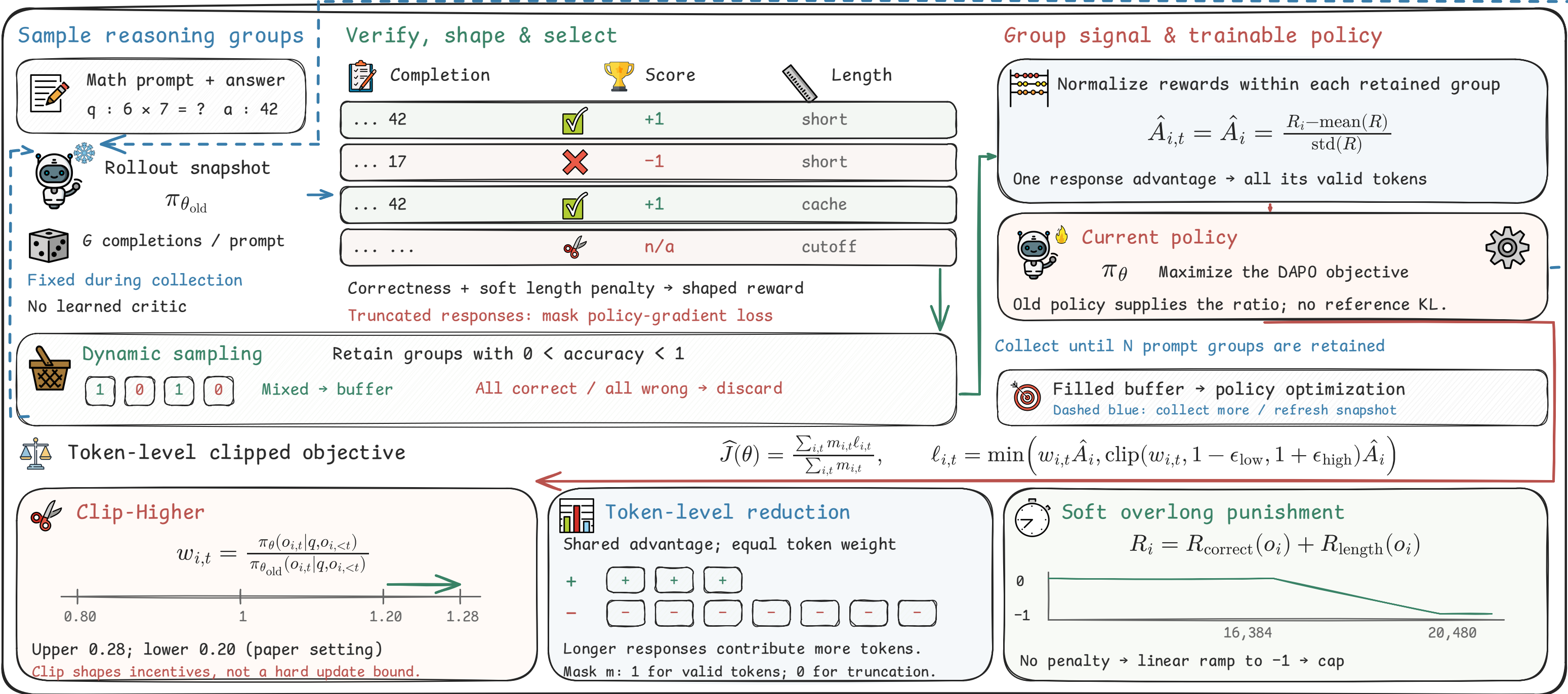
Schematic: four illustrative completions; paper uses G = 16 . Correctness rewards: +1 / -1.
