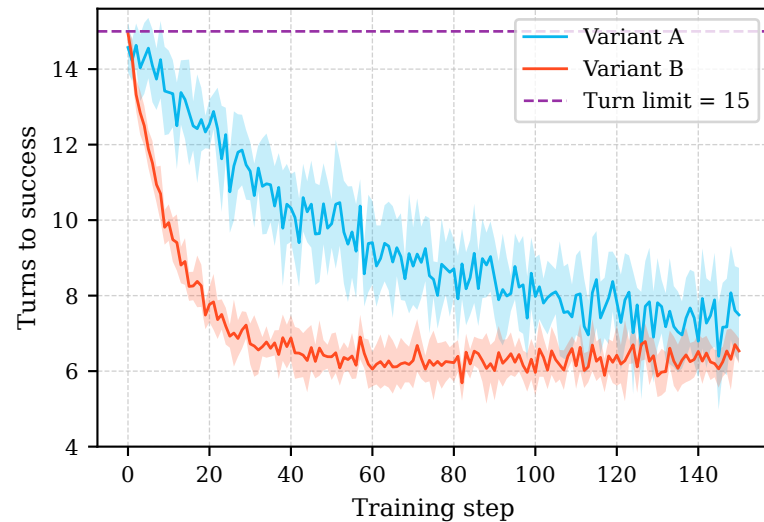
(c) Turn-level efficiency
