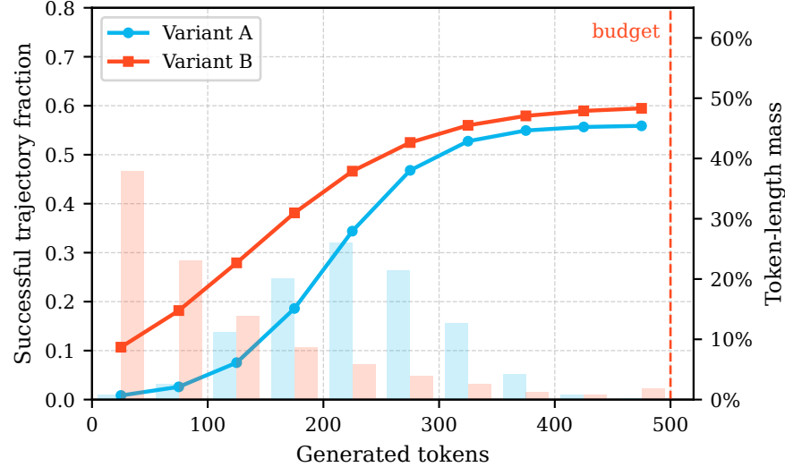
(b) Token-level efficiency
