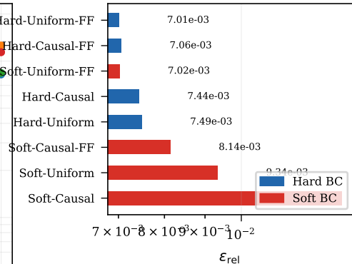
All Burgers variants
