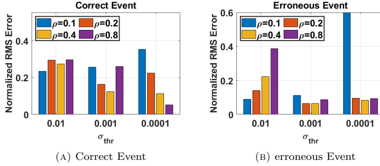
FIGURE 14. Normalized RMS error of ERP prediction using weighted incremental DMD with initial window of 128 samples during (a) correct event, and (b) Erroneous event.
