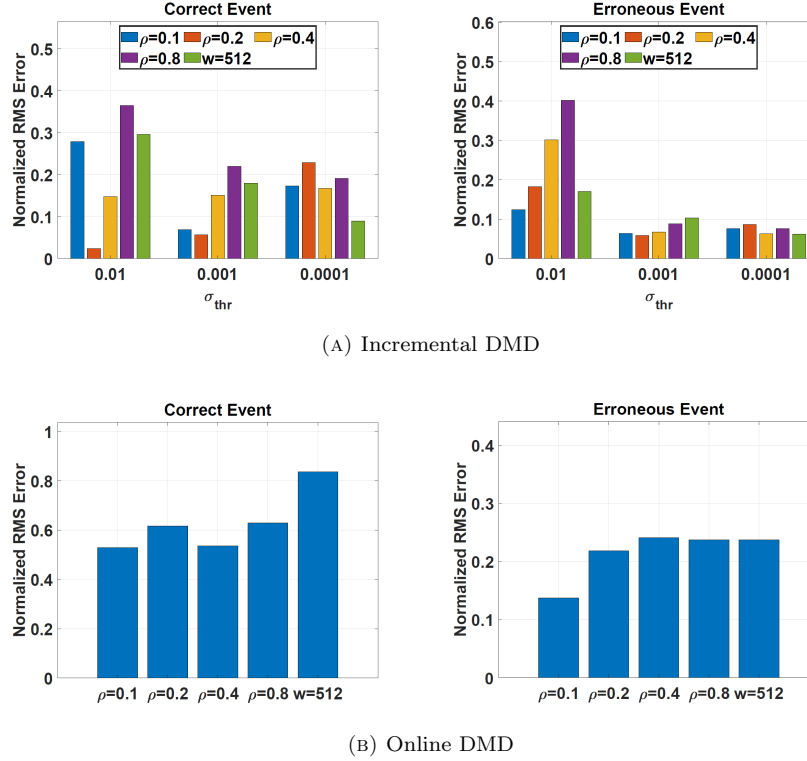
FIGURE 5. Normalized RMS error for the predicted ERP signal at channel FCz for correct events (left panel) and erroneous events (right panel), using (a) incremental DMD, and (b) online DMD.
