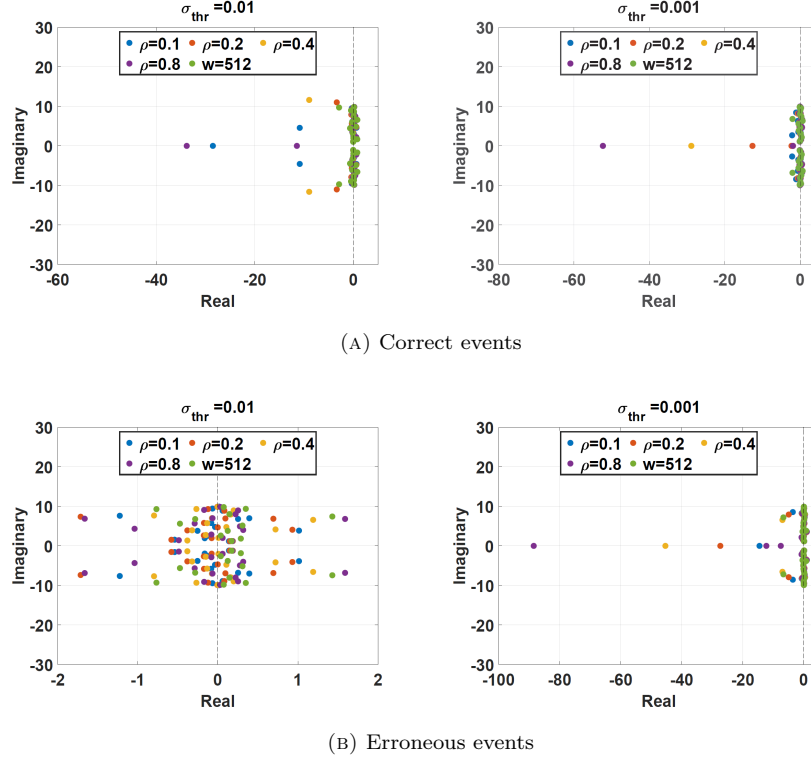
FIGURE 9. The left panel show the continuous time DMD eigenvalues for \sigma_{\text{thr}} = 0.01 and the right panel shows the continuous time DMD eigenvalues for \sigma_{\text{thr}} = 0.001 during (a) correct events (b) erroneous events
