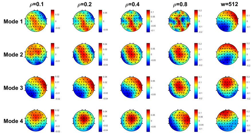
(B) DMD modes \sigma_{\text{thr}} = 0.001 .
