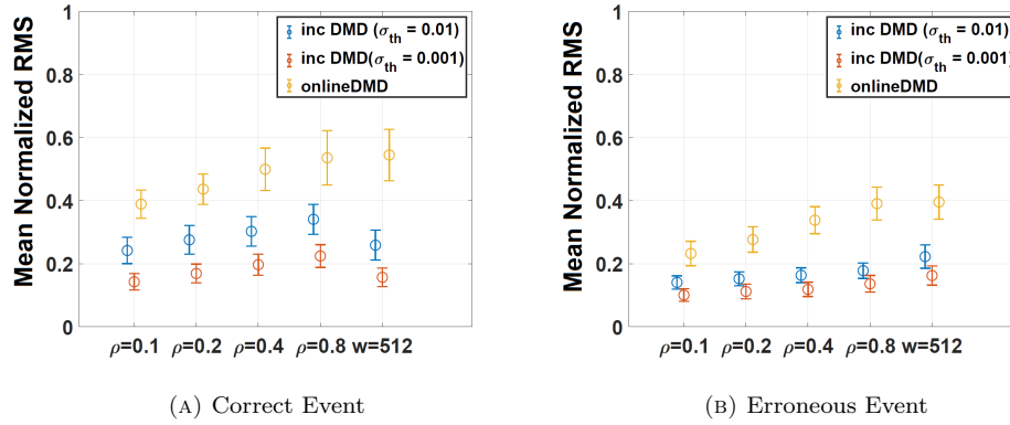
FIGURE 3. The mean of the normalized RMS prediction error computed over all iterations as well as the associated 95% confidence sets for (a) correct events and (b) erroneous events.
