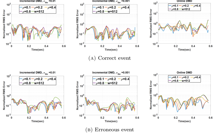
FIGURE 13. Normalized RMS error for a future-window of 64 samples of EEG states at channel FCz using incremental DMD with \sigma_{thr} = 0.01 (left panel), incremental DMD with \sigma_{thr} = 0.001 (middle panel), and online DMD (right panel) for (a) correct event, and (b) erroneous event.
