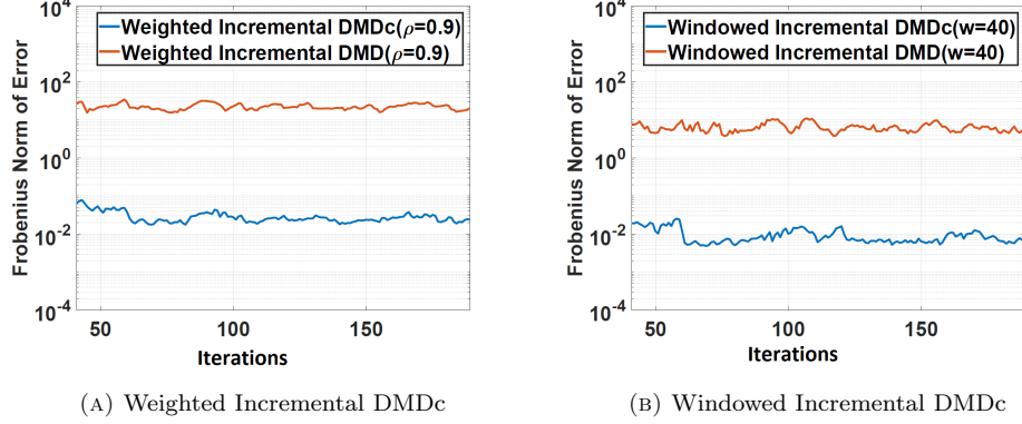
FIGURE 12. The Frobenius norm of prediction error for a future-window of 10 samples using (a) weighted incremental DMD (red line) and weighted incremental DMDc (blue line), and (b) windowed incremental DMD (red line) and windowed incremental DMDc (blue line).
