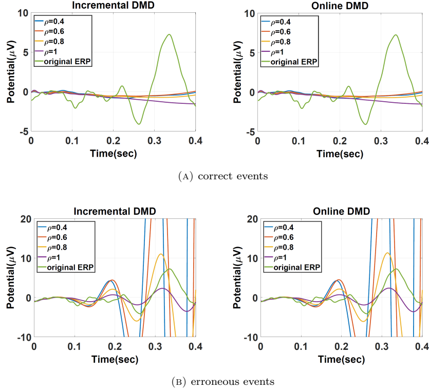
FIGURE 6. The predicted ERP signal at channel FCz based on well conditioned EEG datasets using incremental DMD model (left panel) and online DMD model (right panel) during (a) correct events and (b) erroneous events.
