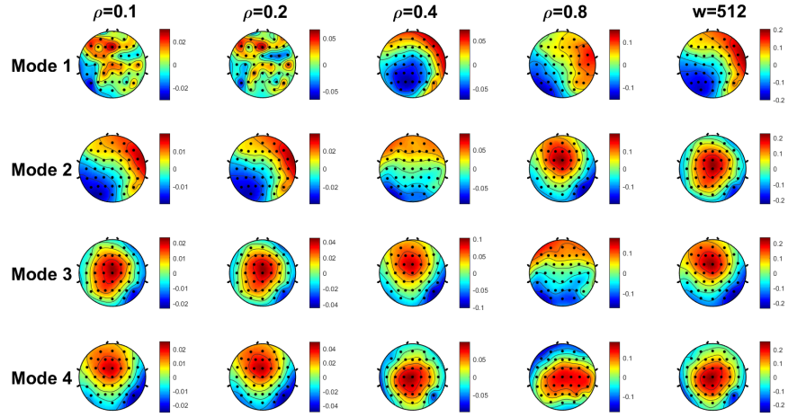
(A) DMD modes \sigma_{\text{thr}} = 0.01 .
