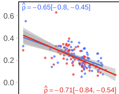
Word Length
