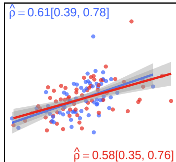
Lexical Frequency
