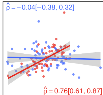
Surprisal
