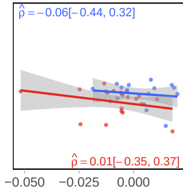
Lexical Frequency
