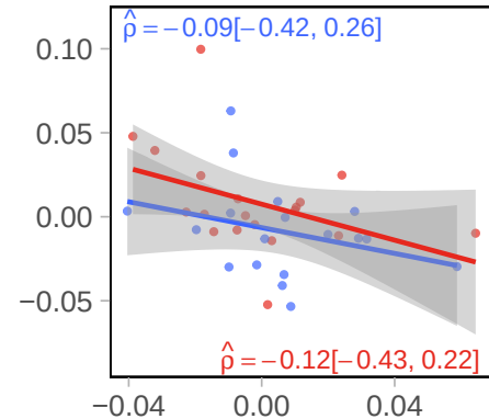
Word Length
