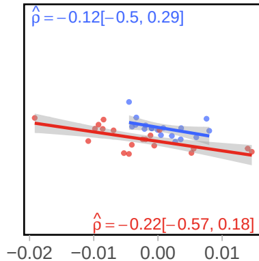
Surprisal
