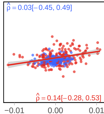
Surprisal
