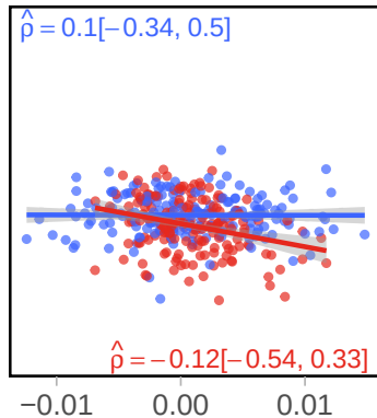
Lexical Frequency
