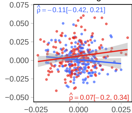
Word Length
