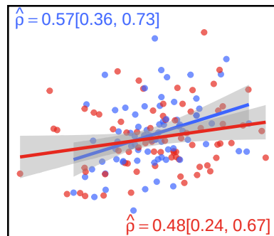
Lexical Frequency
