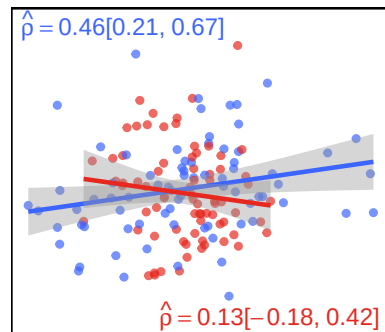
Surprisal
