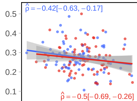
Word Length
