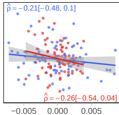
Regression Rate
