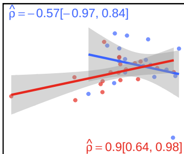
Lexical Frequency
