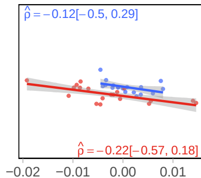
Local Effect
