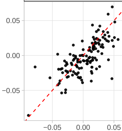
Word Length
