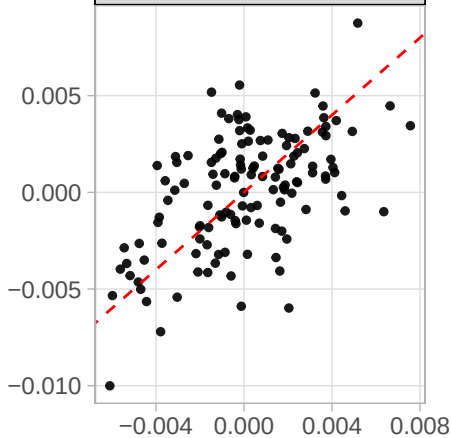
Surprisal
