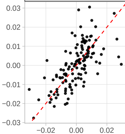
Lexical Frequency
