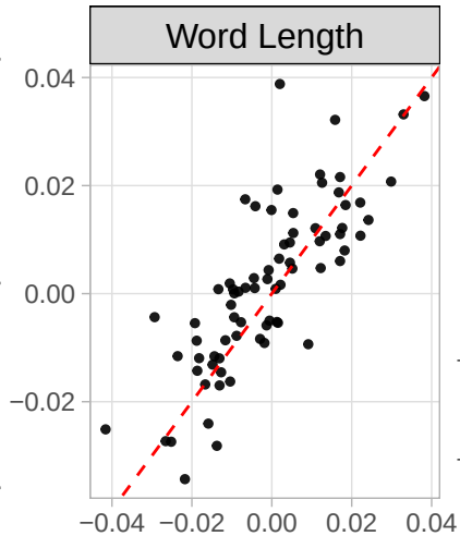
Spillover Effect (Out-of-domain)
