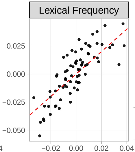
Spillover Effect (In-domain)
