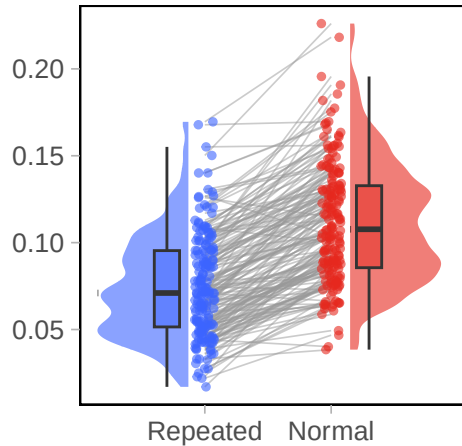
Lexical Frequency
