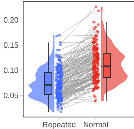
Surprisal
