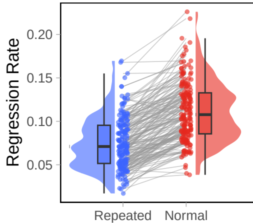
Word Length
