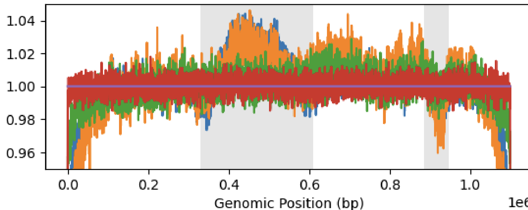
Average Contact Map - 5000 Digestion Bond Cuts
