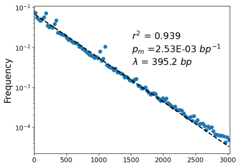
Chromosome 1
