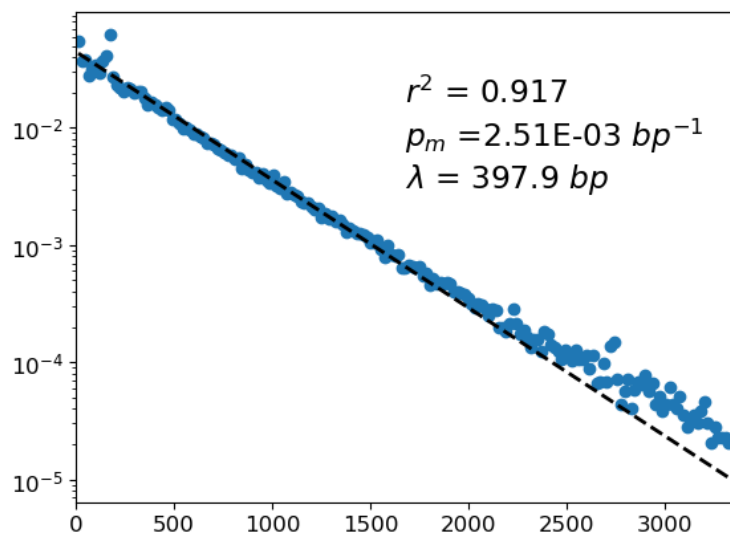
Chromosome 7
