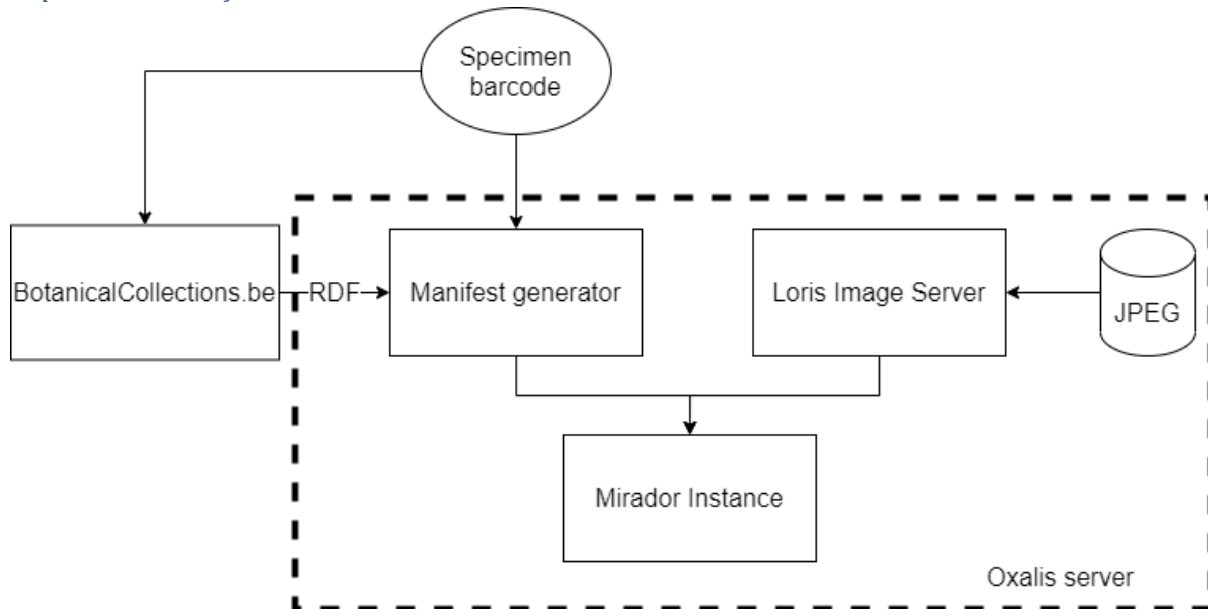
Figure 18: Schematic overview of the current implementation of the IIIF service
