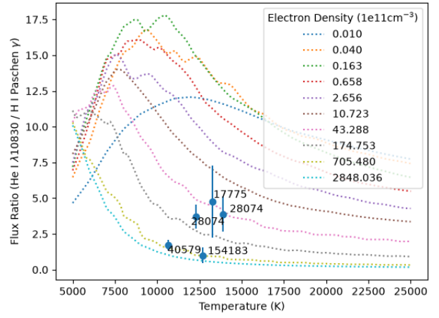
Figure 8. Graph showing which density lines the flux ratios are best approximated by. Density lines are chosen based on a logarithmic scale similar to that of the Pyneb matrix. Here, the LRDs now reveal themselves to be closer to the extreme high-density lines.
