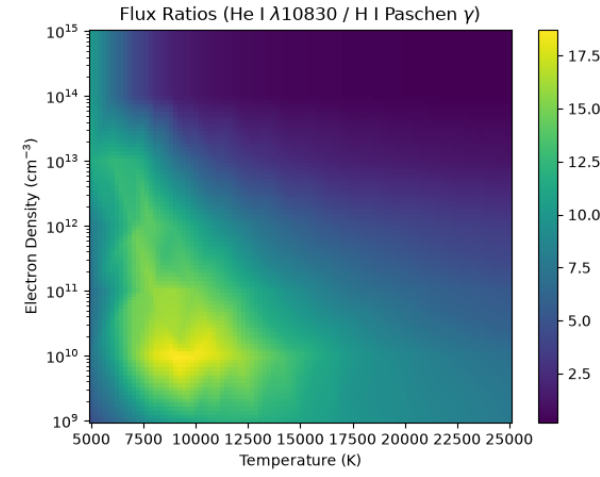
Figure 7. Flux ratio prediction matrix generated by Pyneb, with density scaled logarithmically. Here we see that now only the higher density region has areas of low flux ratio.
