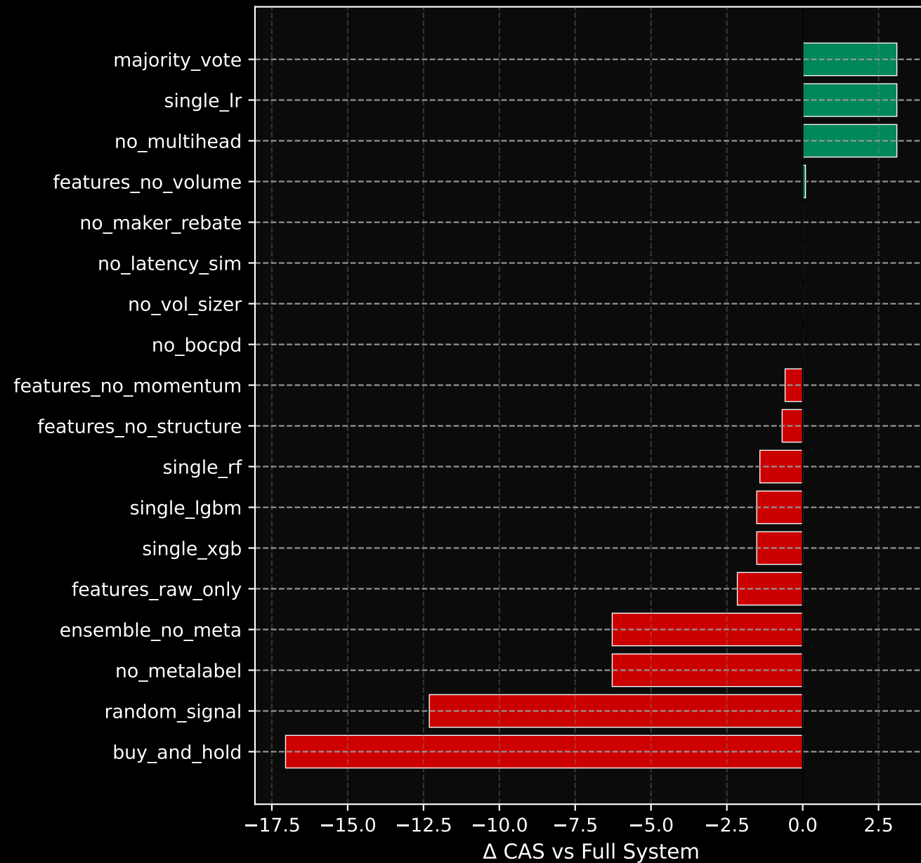
Cost-Adjusted Sharpe Delta
