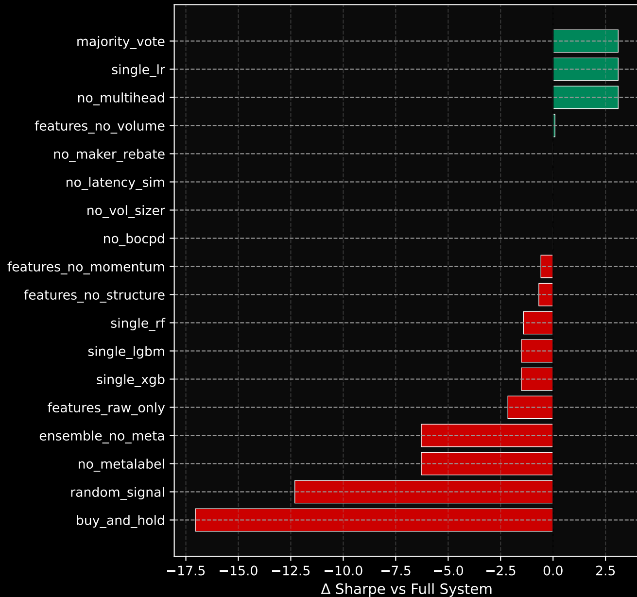
Sharpe Ratio Delta
