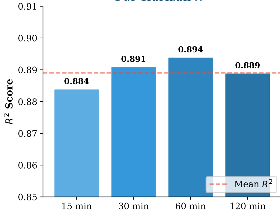
Per-Horizon R^2
