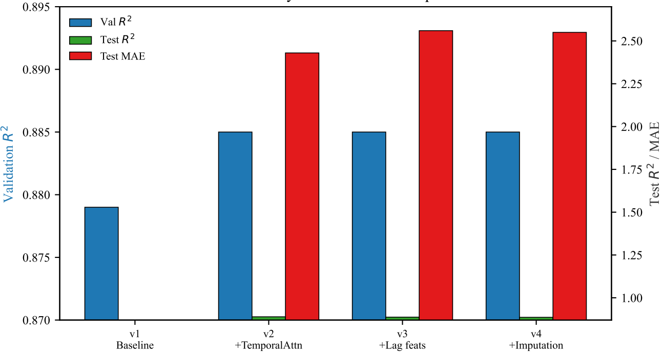
Ablation Study: Architectural Components
